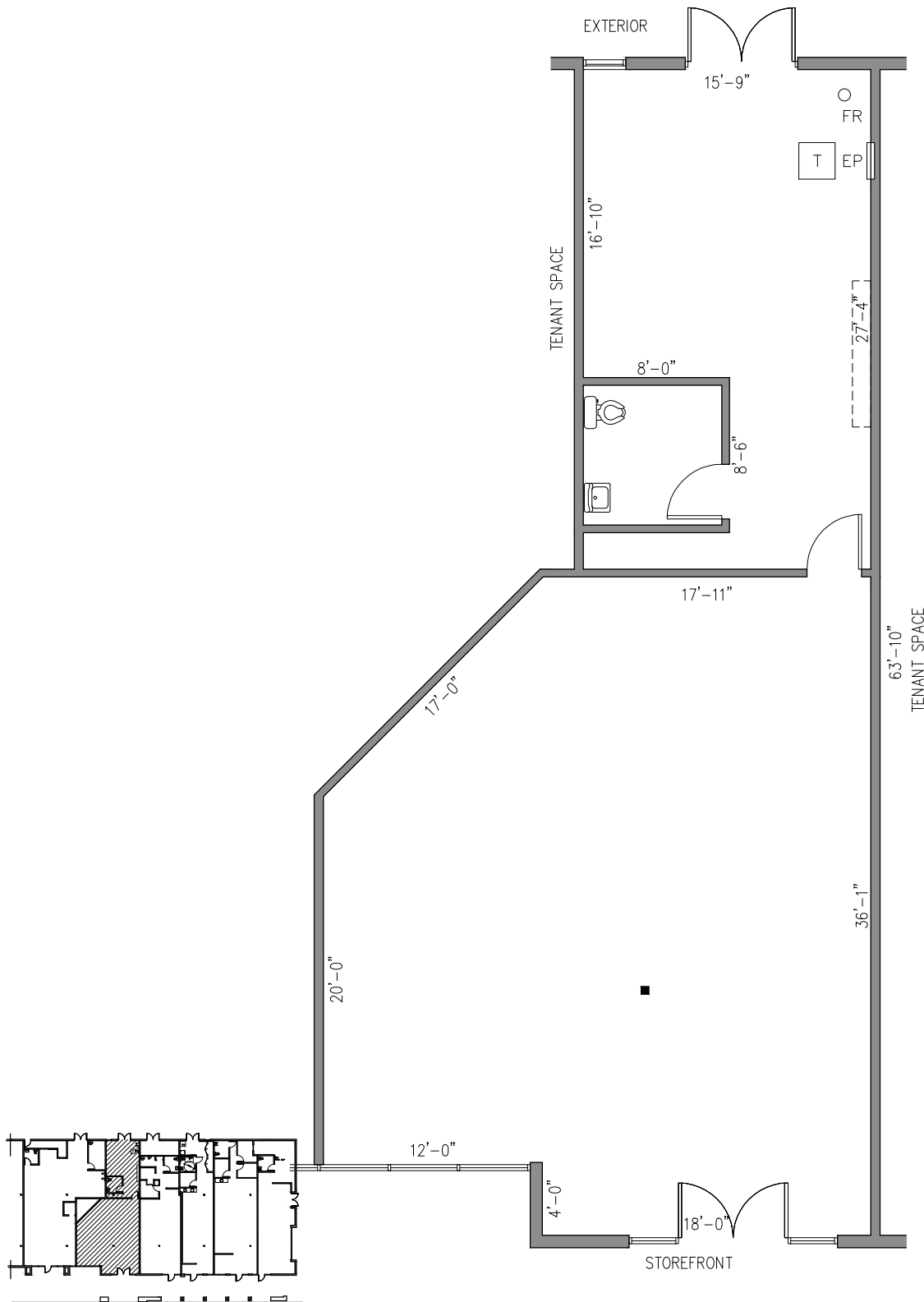
KEY PLAN
