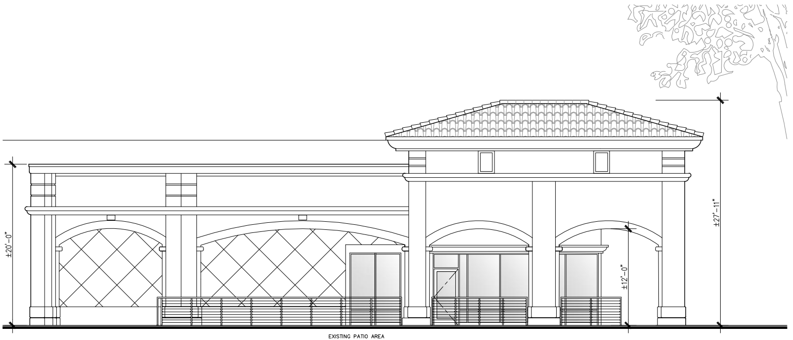
SOUTH ELEVATION
